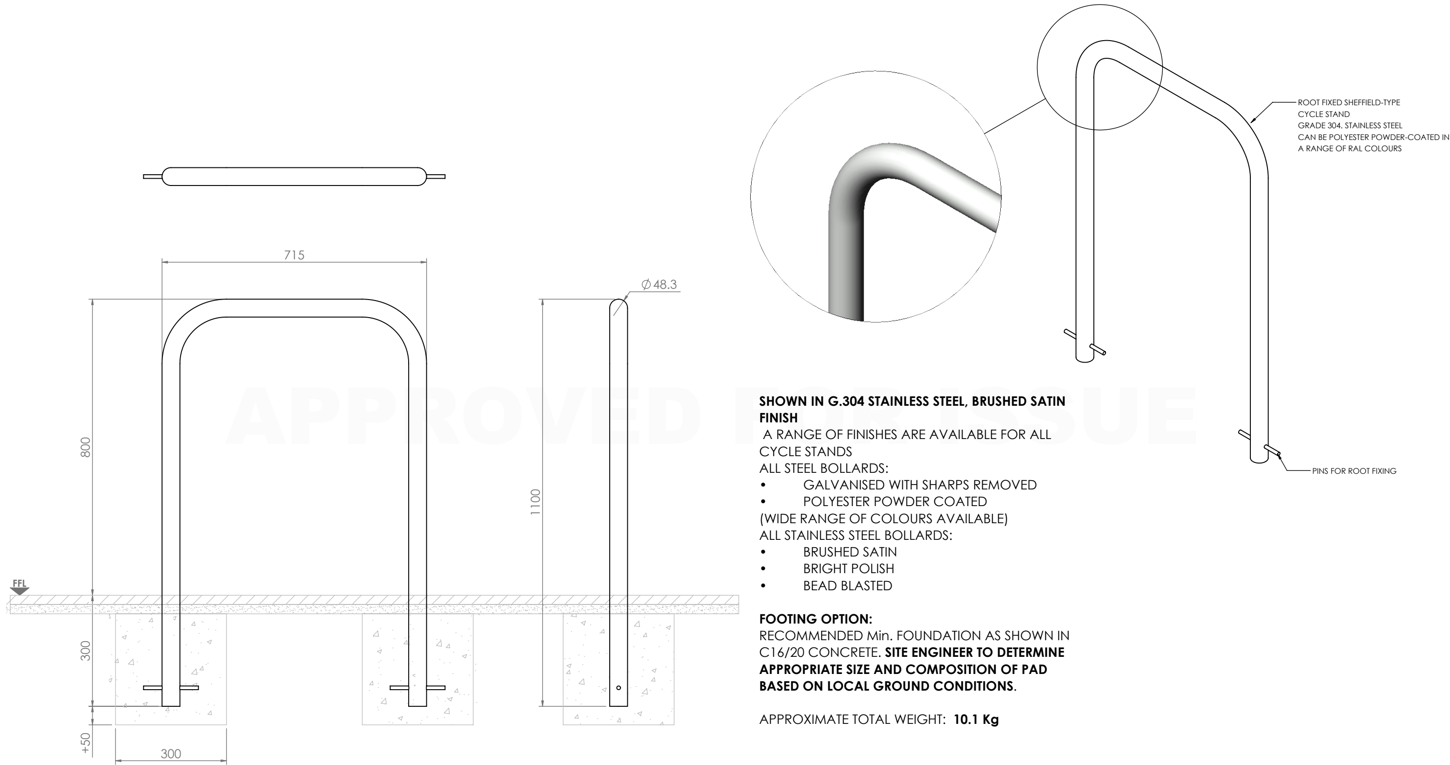
SHEFFIELD CYCLE STAND STAINLESS ROOT FIXED GENERAL ARRANGEMENT
